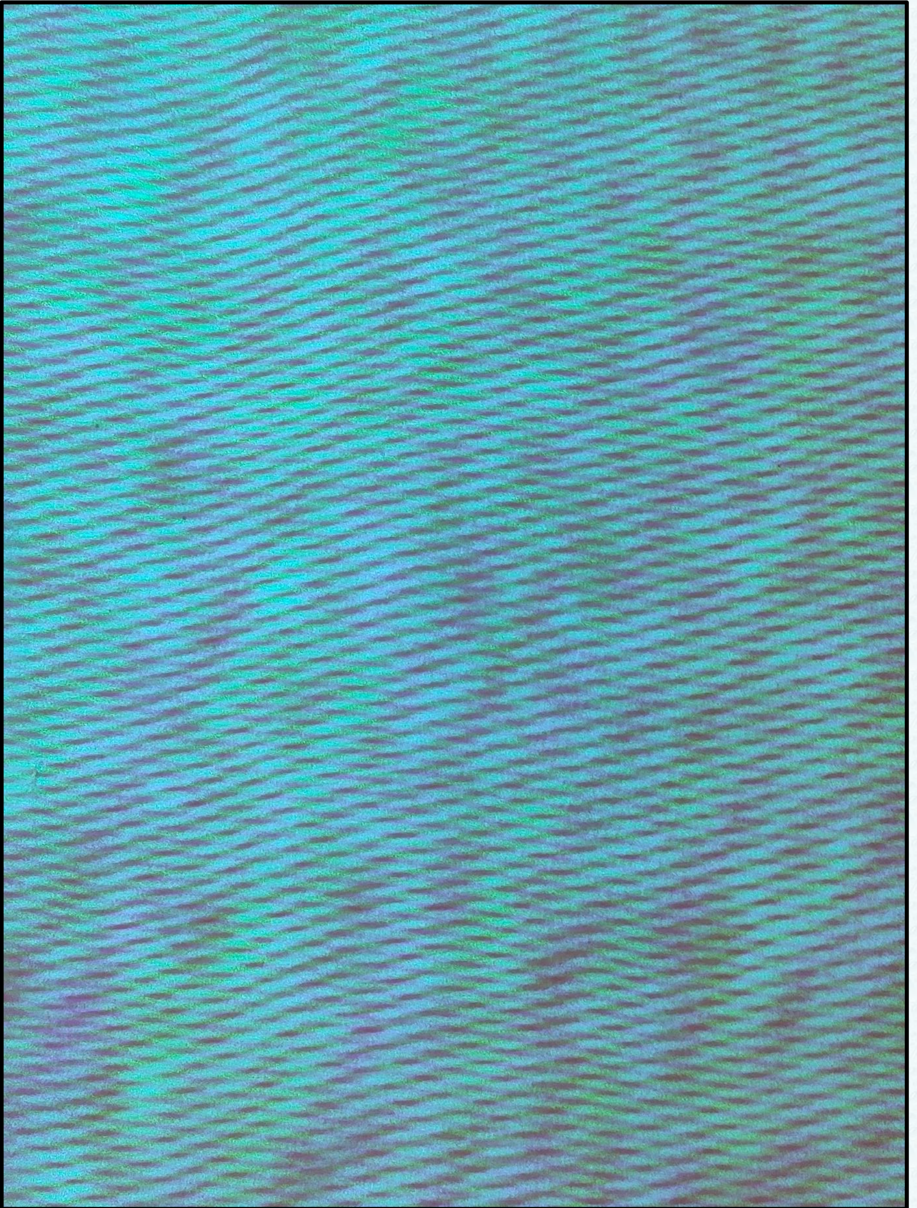
Pavitra Ganapati Bhat. Interferogram using Spatial Heterodyne Spectrometer. The interference pattern (interferogram) from prominent wavelengths in the visible region from the argon ion laser source was recorded using a Spatial Heterodyne Spectrometer and Retiga R1 camera.
